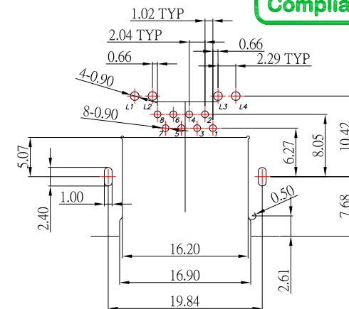
PCB LAYOUT
