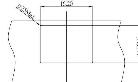
FRONT VIEW RECOMMEND PANEL LAYOUT
